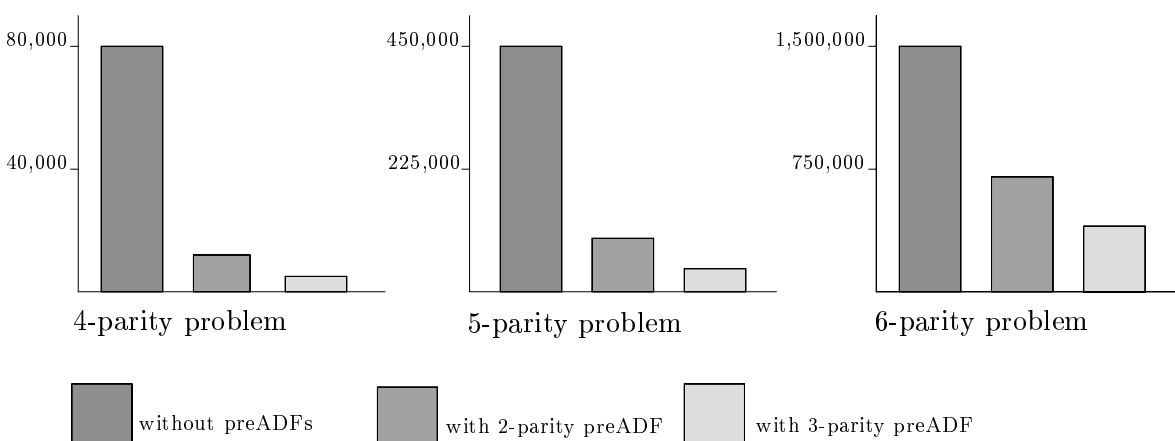
Figure 1: Comparison of the number of fitness evaluations.
