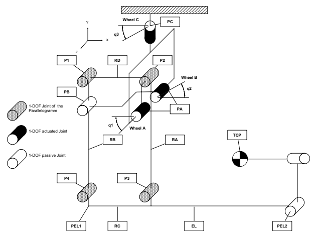
Fig. 2. Kinematic model of the WHI's mechanics
