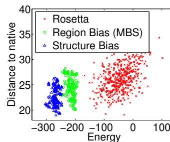
Figure 12: The decoys generated, plotted by their energy and distance to the native structure for Glyceral Kinase (1O0U, 410aa).
